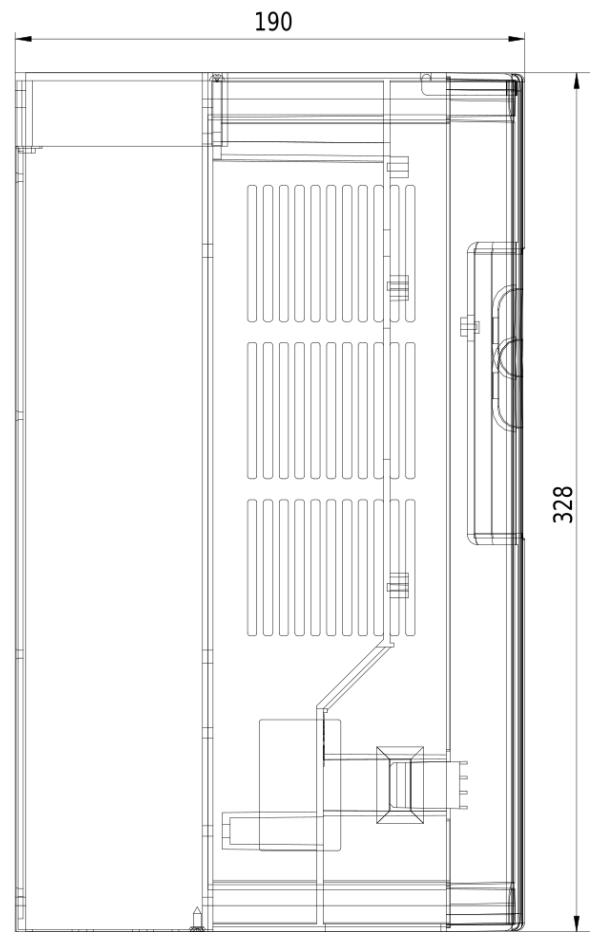
Dimensional drawing V810 - 18,5kW 4T0185
