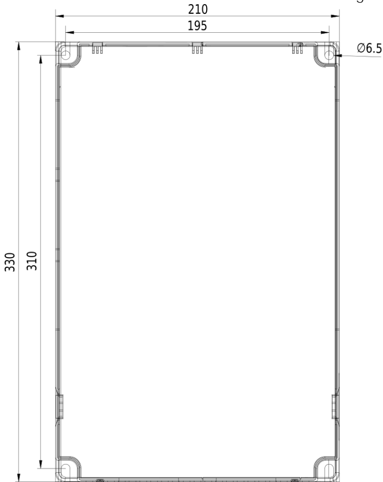
Dimensional drawing V810 - 18,5kW 4T0185
