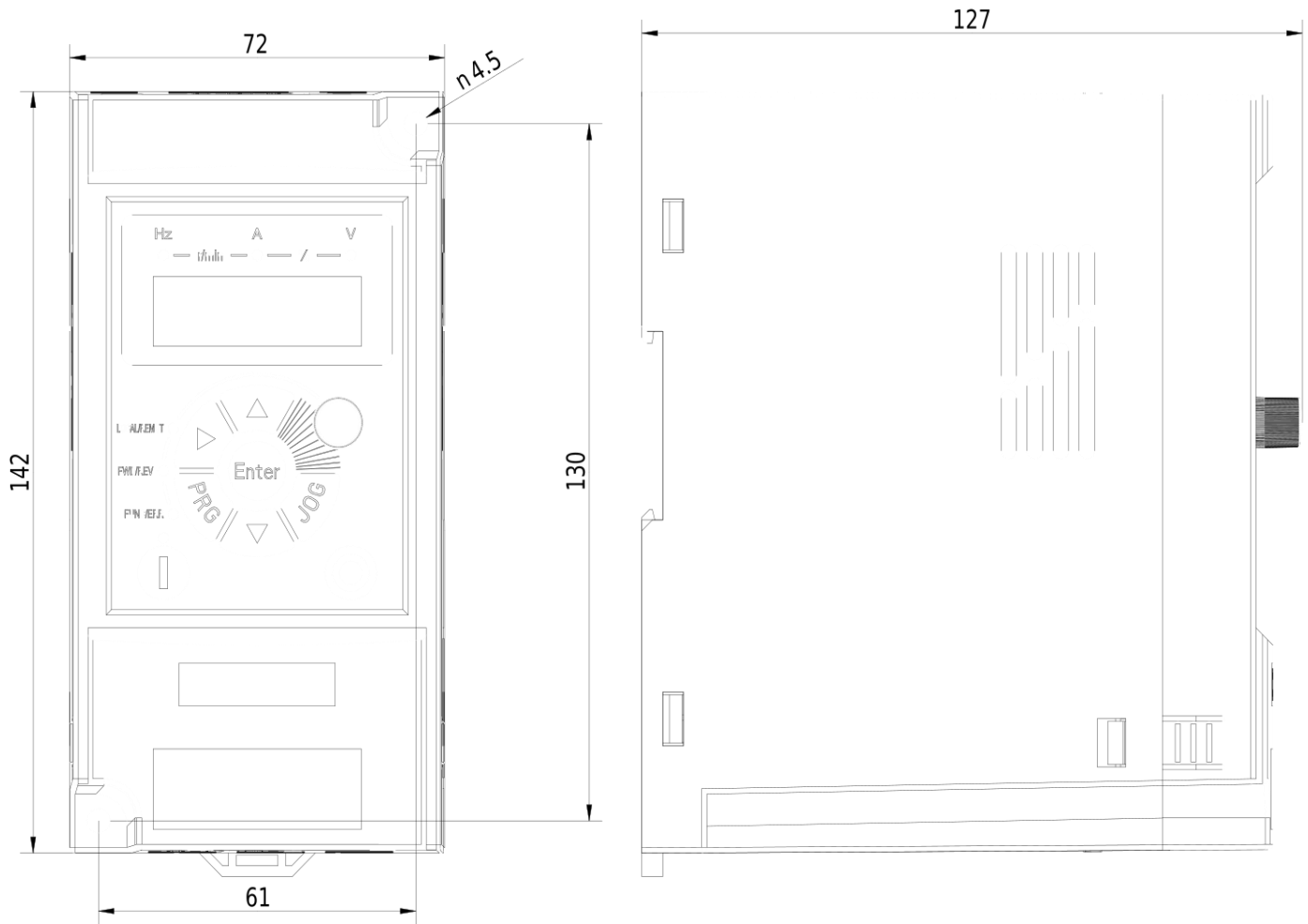
Dimensional drawing V900 - 0,75kW 4T0007
