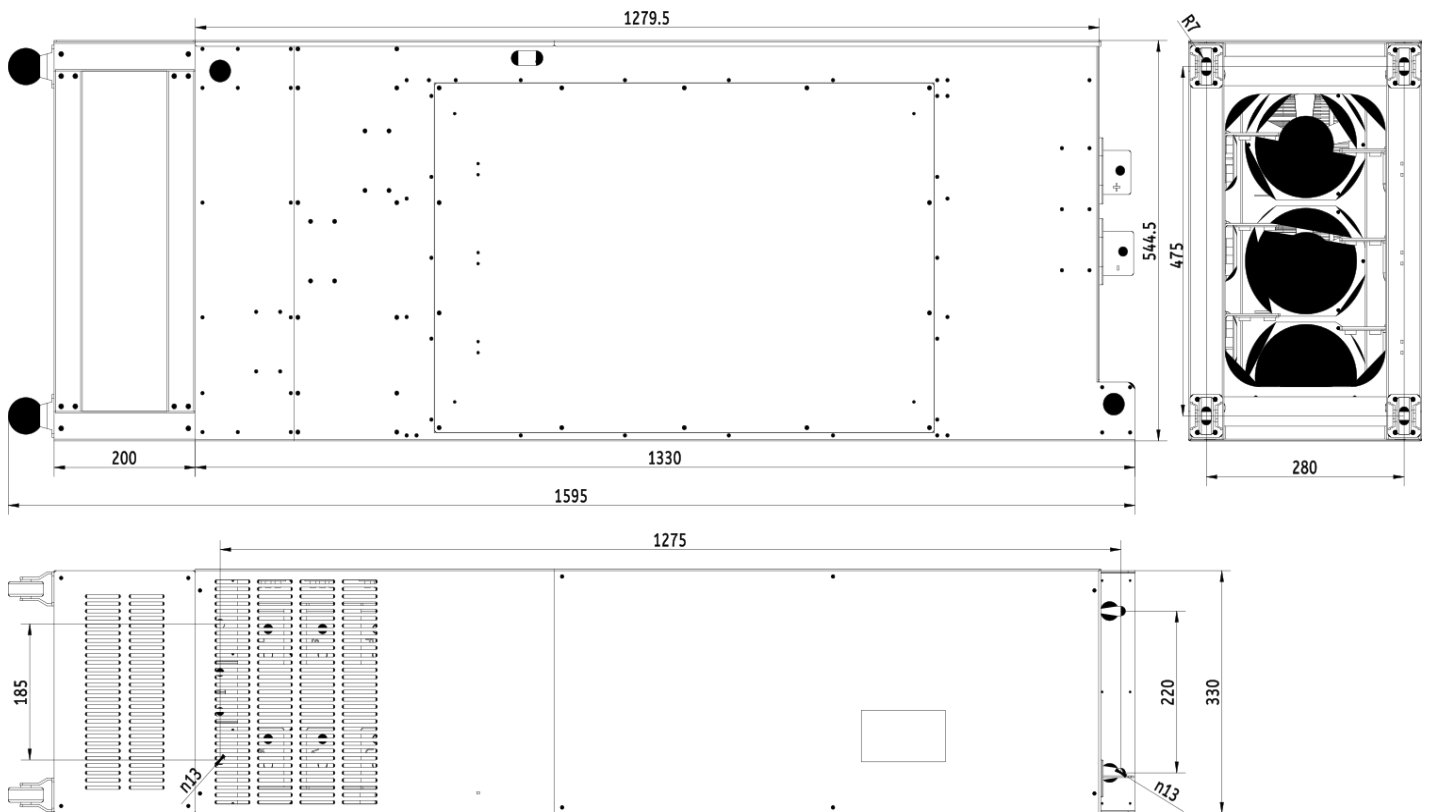
Dimensional drawing V900 - 280kW 4T2800
